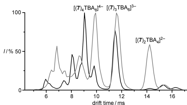
Figure 3. Comparison of the drift time graphs of the main envelope ( m/z = 2305\text{--}2320 \text{ Da} ) for the native compound 7 (black) and after UV irradiation (gray). The spectra were consistent for all three repeated cycles.
